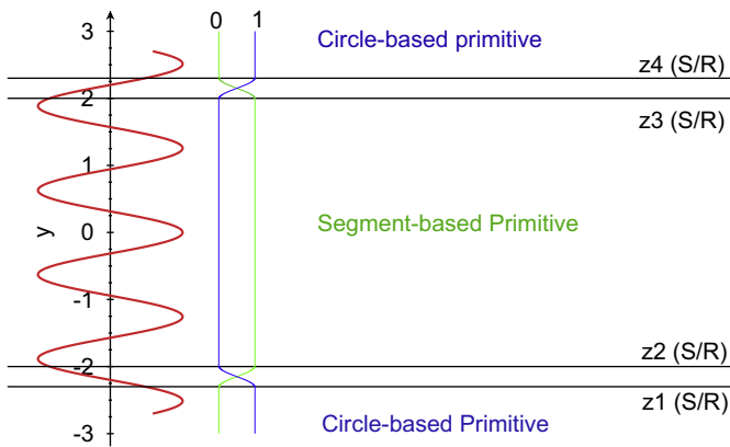
Fig. 13. Transition between the two kinds of primitives in function of S/R .
