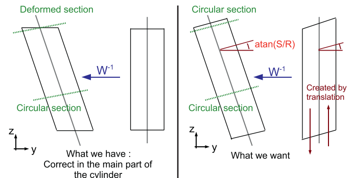
Fig. 12. Idea justifying the correction of both ends of the primitive.
