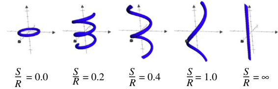
Fig. 2. Shape of the helix for increasing value of S/R .
