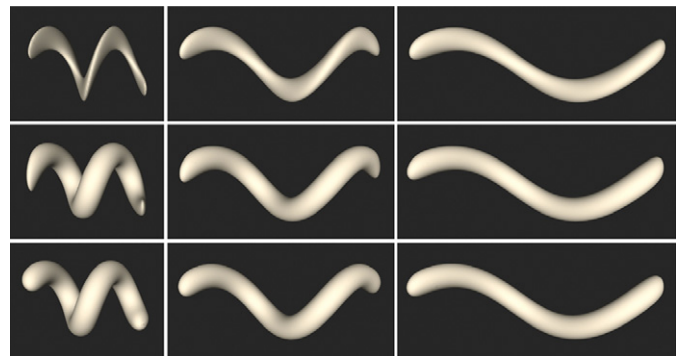
Fig. 10. Comparison, for different values of S/R , between the classic twist (first row), the solution with the end point problem (second row) and our final solution (third row).
