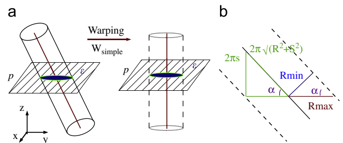
Fig. 9. (a) Transformation W_{\text{simple}} applied to an inclined cylinder. (b) Lateral view of that cylinder.
