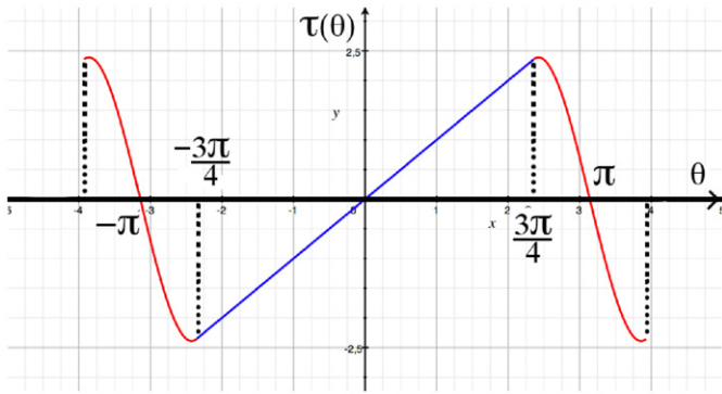
Fig. 6. Amount of translation along the z -axis according to the angle \theta in cylindrical coordinates.
