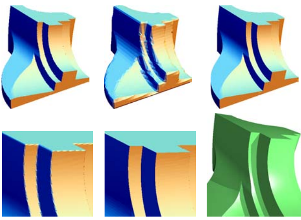
Figure 7: Visualization of the fandisk model implicitized with MPU. Top left: Bloomenthal polygonization was used; in spite of sufficiently high polygonization resolution (200K triangles) one can notice small aliasing defects along sharp features. Top middle: a low resolution polygonization is applied. Top right: an optimized mesh (17K triangles) is obtained from the low resolution mesh, the sharp features are accurately reconstructed. Bottom left: a magnified part of the high resolution mesh. Bottom middle: the same part of the optimized mesh. Bottom right: a part of the model rendered using Hart sphere tracing.
